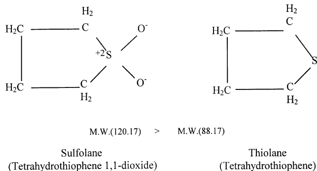
Fig. 1. Structural formula of sulfolane and thiolane used for oxygen-uptake characteristics on a soil microcosm.
